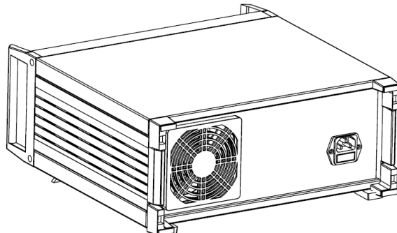
BACK VIEW
